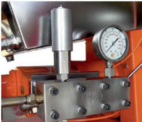
Stainless steel Pump Head
