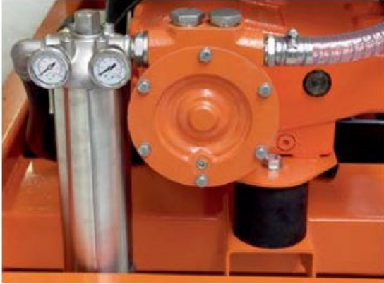
Built-on mechanical feed pump
